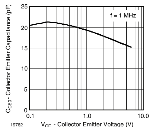
Fig. 5 - Collector Emitter Capacitance vs. Collector Emitter Voltage
